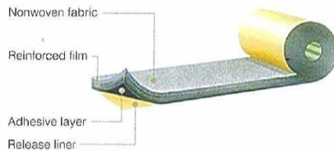
Structure (single-coated adhesive type)
