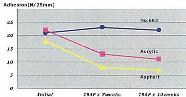
194F x 14Weeks accelerated test is assumed to be equivalent to 20 Years.
