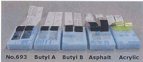
No.693 shows heavy cohesion failure upon removal.
