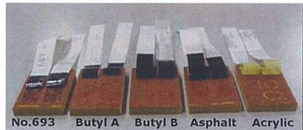
No.693 shows heavy cohesion failure upon removal.
