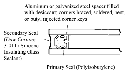
Figure 1: Dual-seal Type
